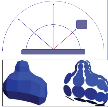
Bottom image credit: "GPU Gems 2", nVidia, 2005. Vertices mapped to illumination disks for hemispheric illumination mapping. 169
