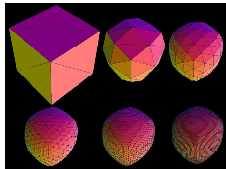
Loop subdivision in action. The asymmetry is due to the choice of face diagonals. Image by Matt Fisher, http://www.its.caltech.edu/~matthewf/Chatter_Subdivision.html
