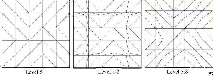
Level 5
