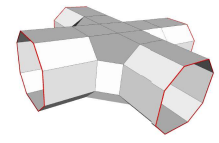
(1) 54 faces
