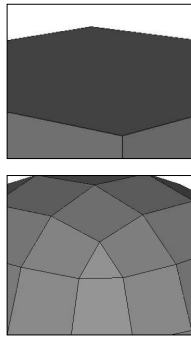
Detail of Doo-Sabin at cube corner
