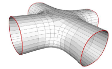
(3) 702 faces
