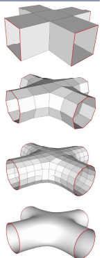
(Catmull-Clark in action)
