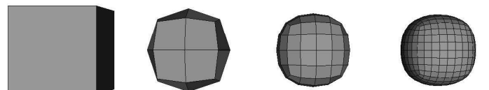
Catmull-Clark
