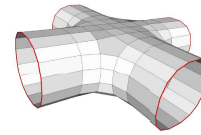
(2) 190 faces
