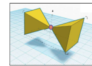
Non-manifold vertex
