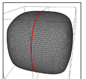
(Top) 5x Catmull-Clark subdivision of a cube (Bottom) 5x Catmull-Clark subdivision of two halves of a cube; the limit surfaces are clearly different.
